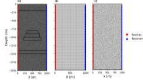
Fig. 3. (a) Geometric framework of the forward modeling mesh, delineating the subsurface discretization for wave propagation across the survey domain; (b) Structured inversion mesh configuration, illustrating a uniform grid-based discretization optimized for inversion stability; (c) Unstructured inversion mesh layout, showcasing an adaptive triangular discretization tailored to enhance resolution of subsurface features.
