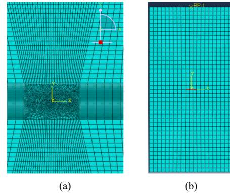
Fig. 16. (a) Stationary Mesh, (b) XFEM Mesh.
