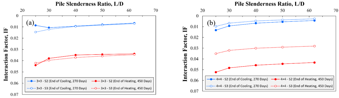
Fig. 13 Influence of pile slenderness ratio ( L/D ) on interaction factor for two pile spacings ( S = 2 m and 3 m): a 3 \times 3 energy pile group, b 4 \times 4 energy pile group
