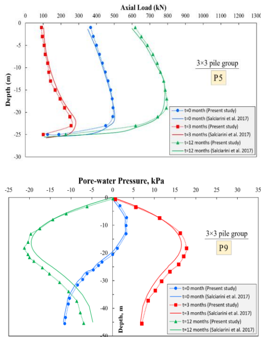
Fig. 6. Energy pile group response verification for the 3 × 3 pile group: a axial load distribution with depth for pile P5, b pore-water pressure distribution with depth for pile P9
