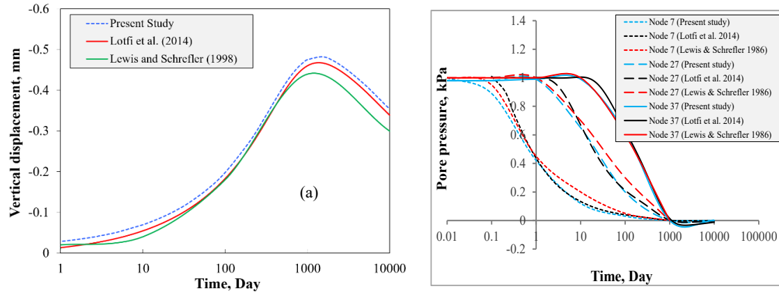
Fig. 3. Thermal consolidation verification: a vertical displacement–time response, b pore-water pressure dissipation at selected monitoring nodes
