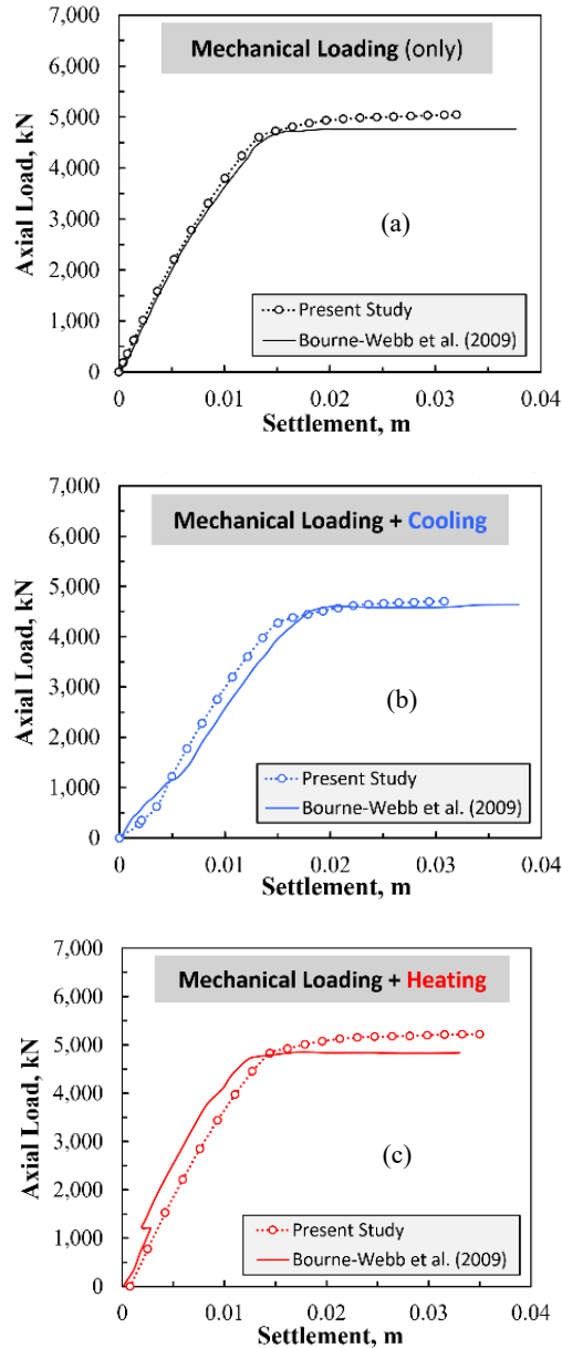
Fig. 5. Full-scale single energy pile validation based on axial load–settlement response under: a mechanical loading, b mechanical loading with cooling, c mechanical loading with heating
