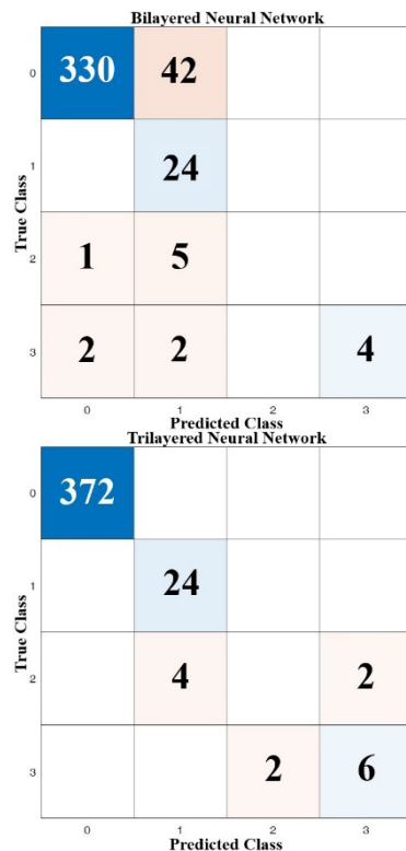
Figure 6. Neural Networks multi-class classification results
