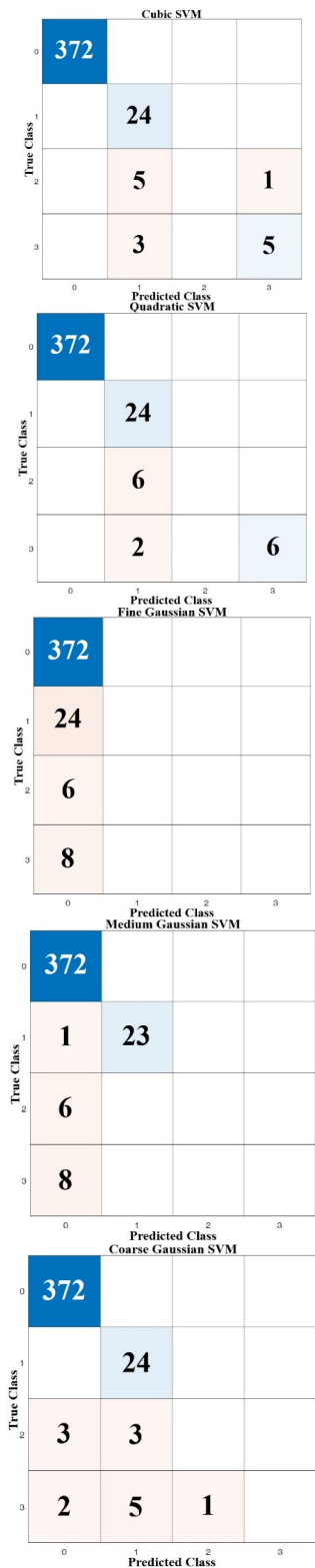
Figure 5. Support Vector Machine multi-class classification results
