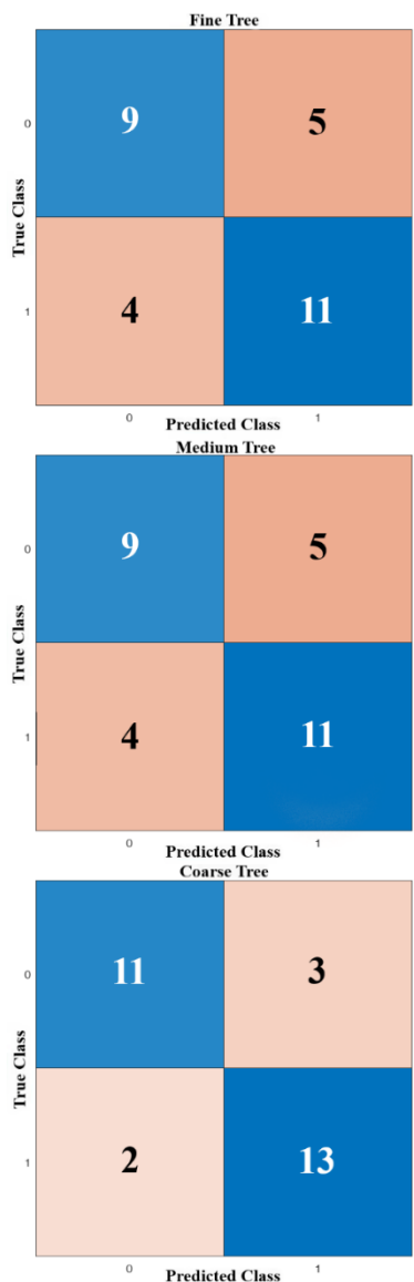
Figure 1. Decision Tree binary classification results
