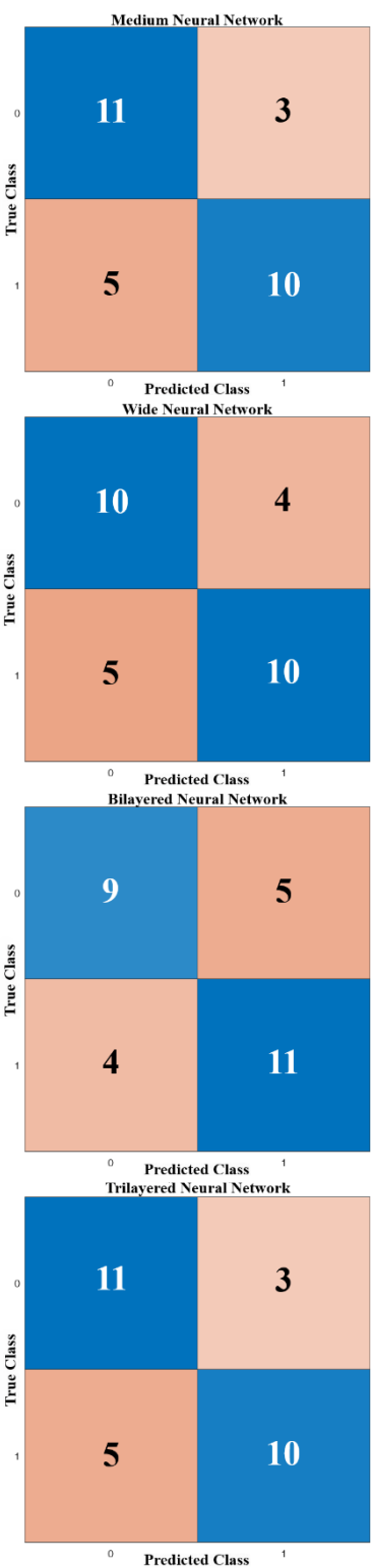
Figure 3. Neural Networks binary classification results
