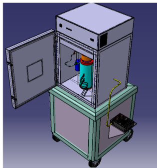
Fig. 2. CAPRI system designed in Catia software
